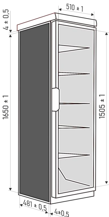
Branding scheme (in mm)
